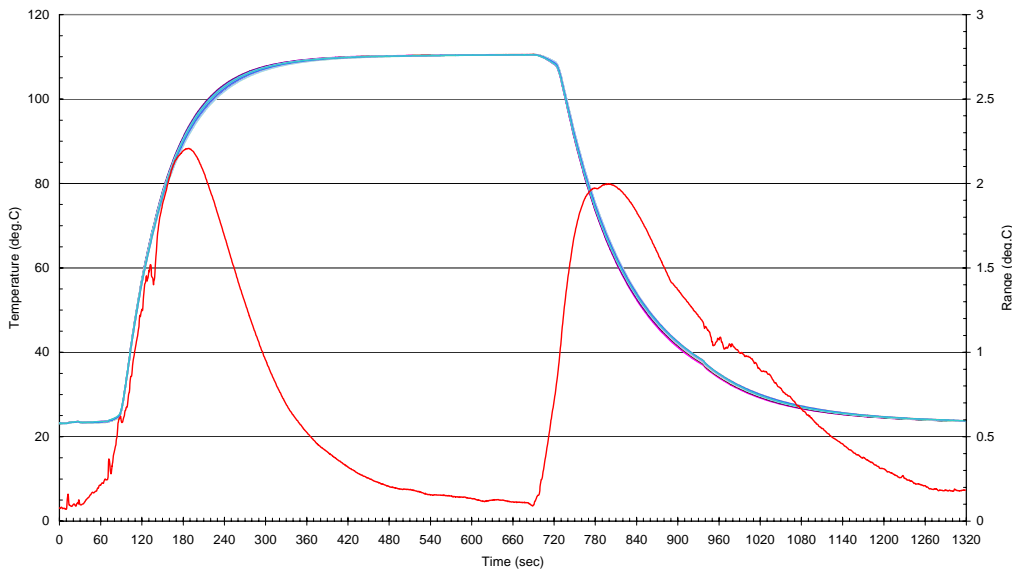
AccuTemp - 110degC-Heater & 23degC-Cooler
